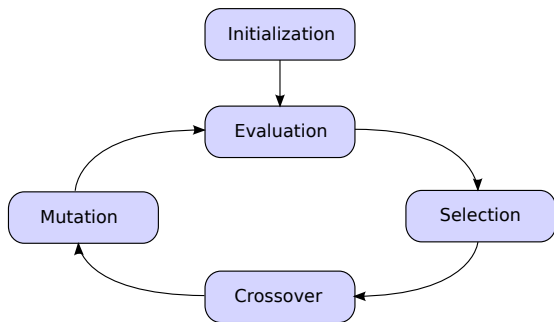
Fig. 3: GA flowchart.
